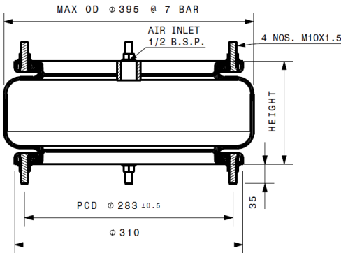
Section View
