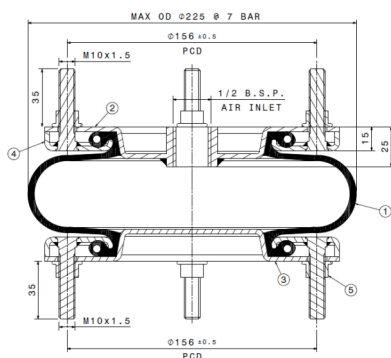
Section View
