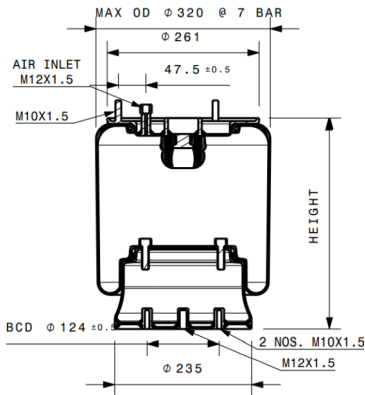
Section View
