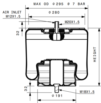
Section View
