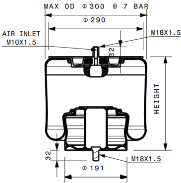
Section View
