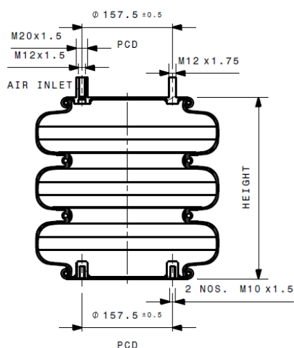
Section View
