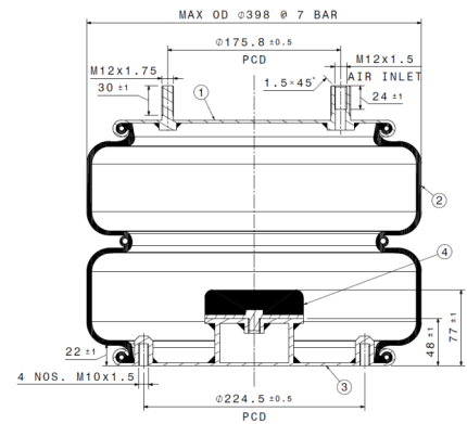
Section View
