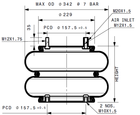
Section View
